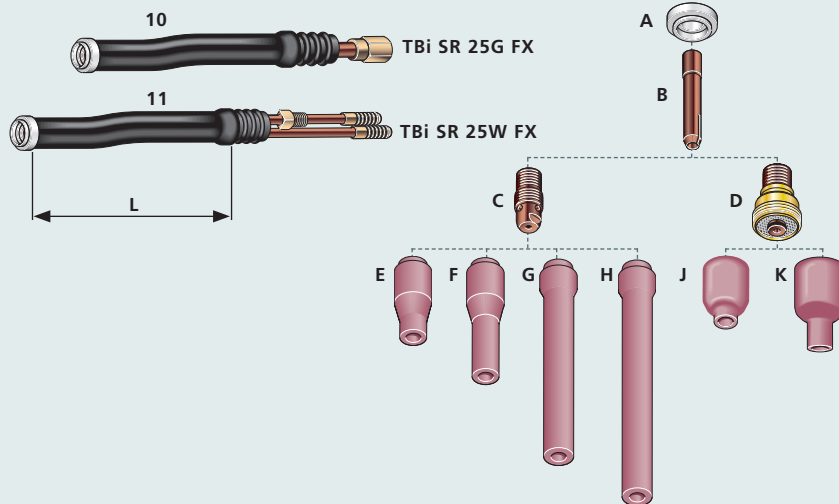
TBi SR 25G FX / TBi SR 25W FX
